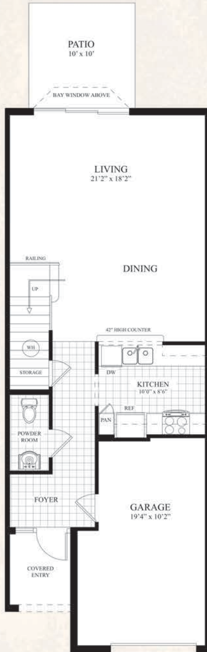
1ST FLOOR
